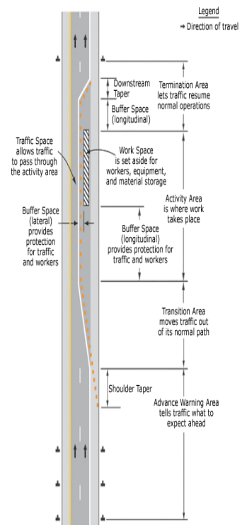
Figure 1. Component Parts of a Temporary Traffic Control Zone
